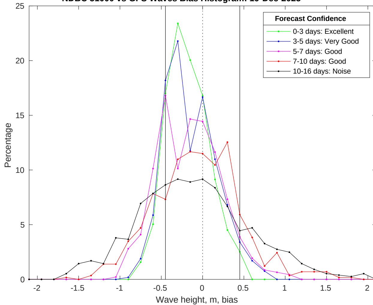
NDBC 51000 vs GFS Waves Bias Histogram: 19-Dec-2025
