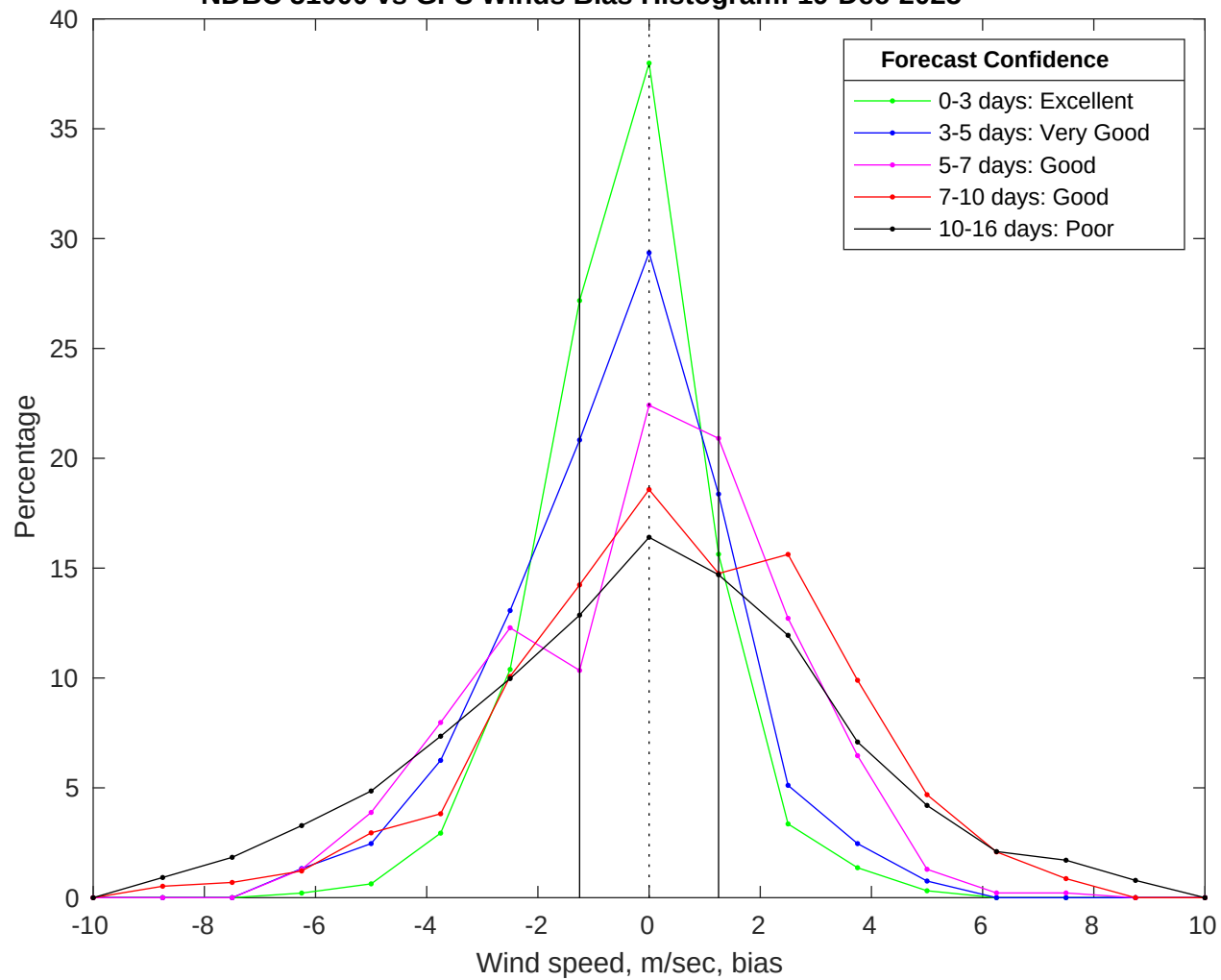
NDBC 51000 vs GFS Winds Bias Histogram: 19-Dec-2025
