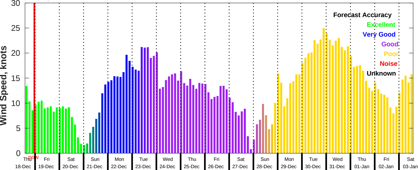
GFS Wind Speed Forecast for NDBC 51000 from 18-Dec-2025 14:00:00 to 03-Jan-2026 14:00:00
