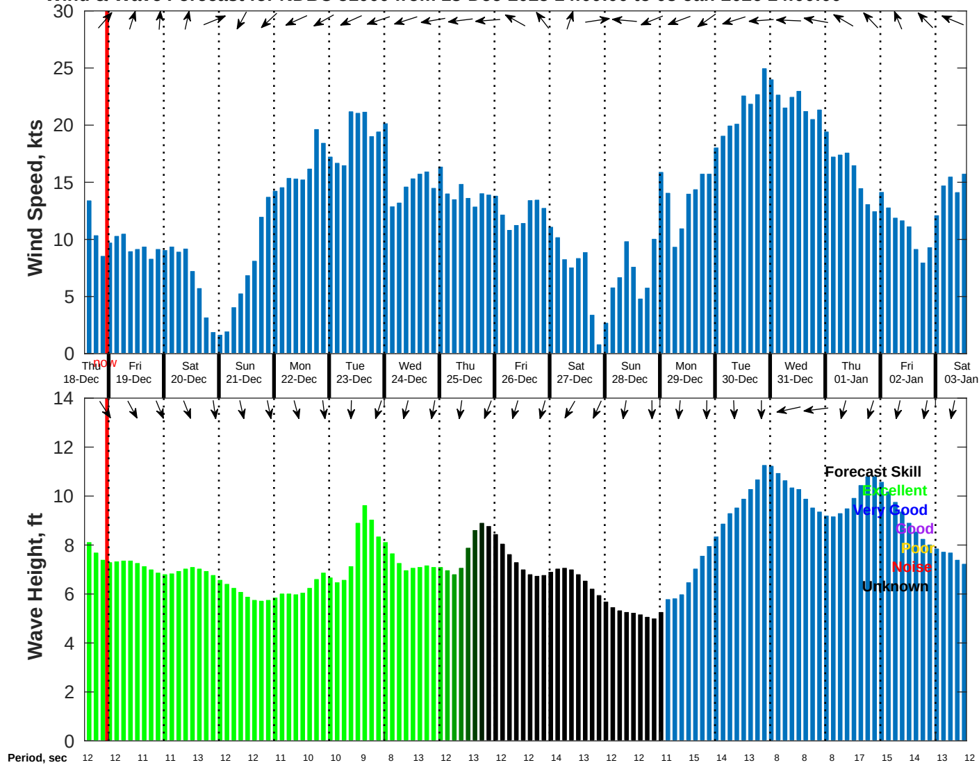
Wind & Wave Forecast for NDBC 51000 from 18-Dec-2025 14:00:00 to 03-Jan-2026 14:00:00
