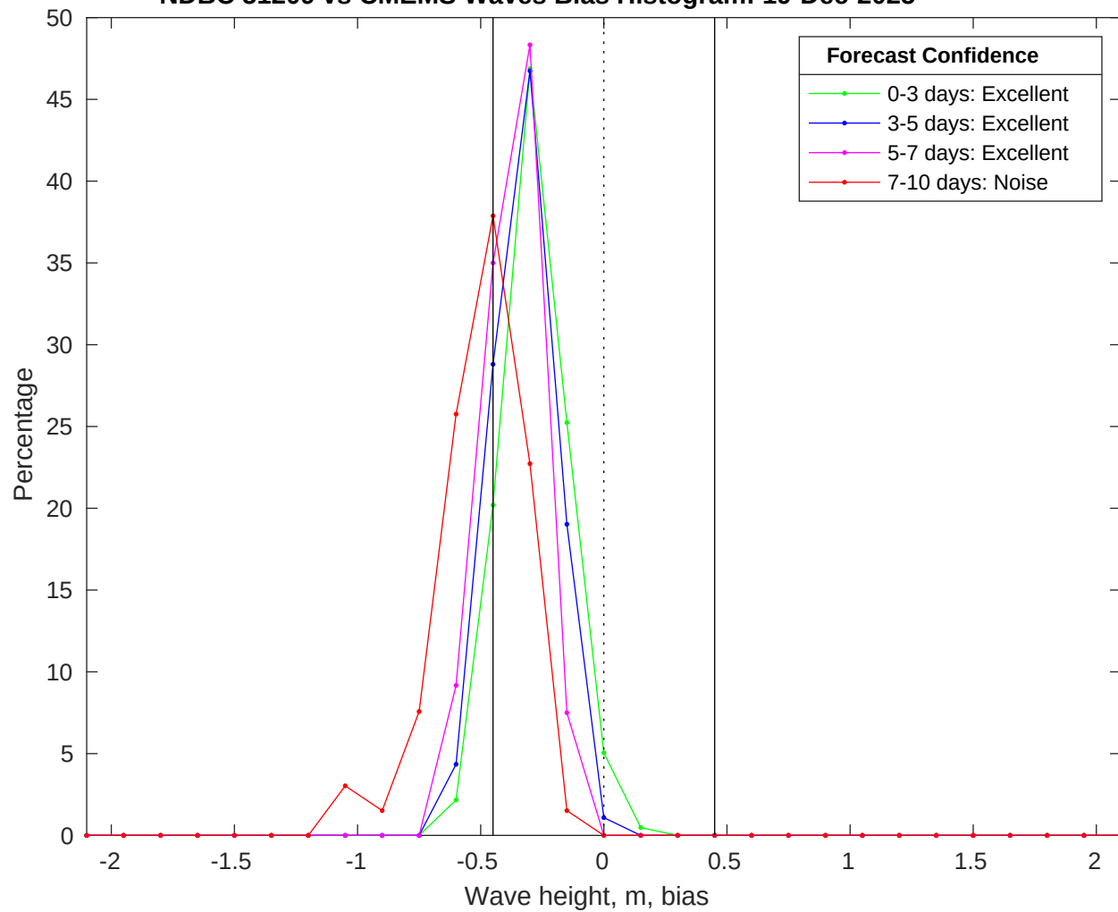
NDBC 51209 vs CMEMS Waves Bias Histogram: 19-Dec-2025
