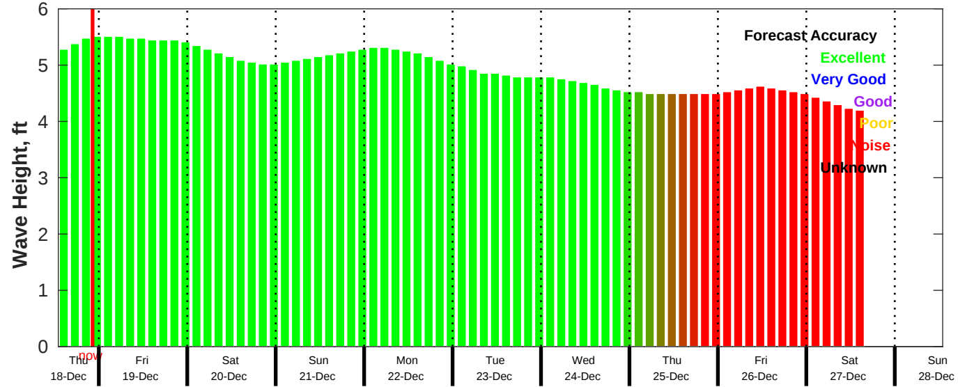
CMEMS Wave Forecast for NDBC 51209 from 18-Dec-2025 13:00:00 to 28-Dec-2025 13:00:00
