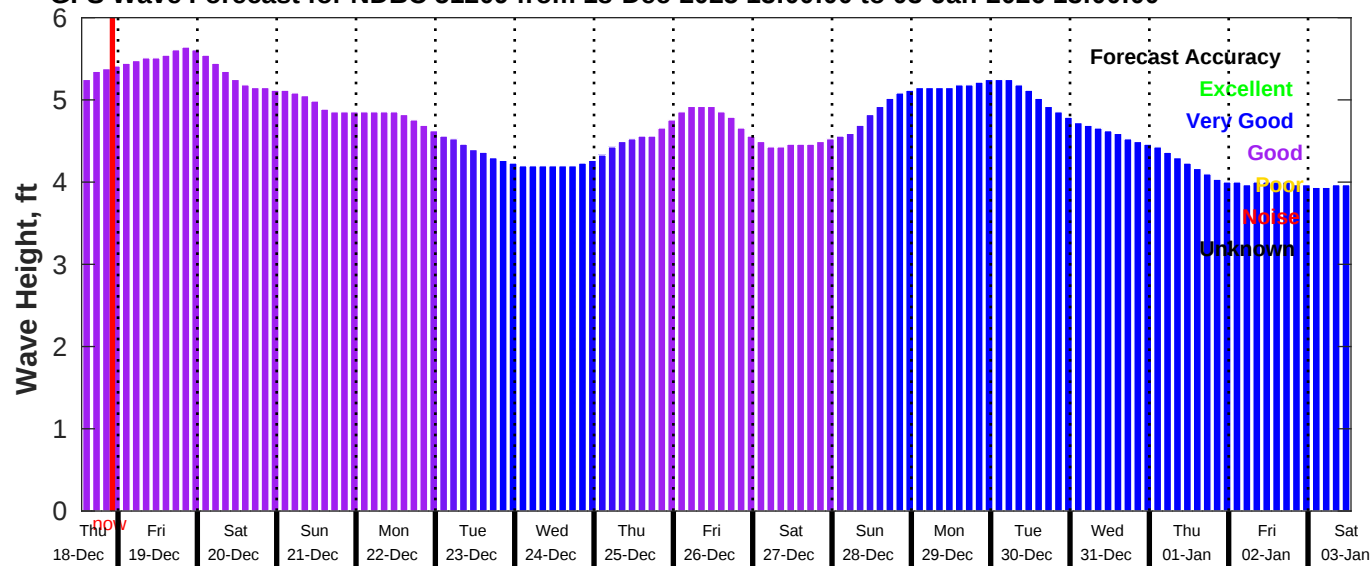
GFS Wave Forecast for NDBC 51209 from 18-Dec-2025 13:00:00 to 03-Jan-2026 13:00:00
