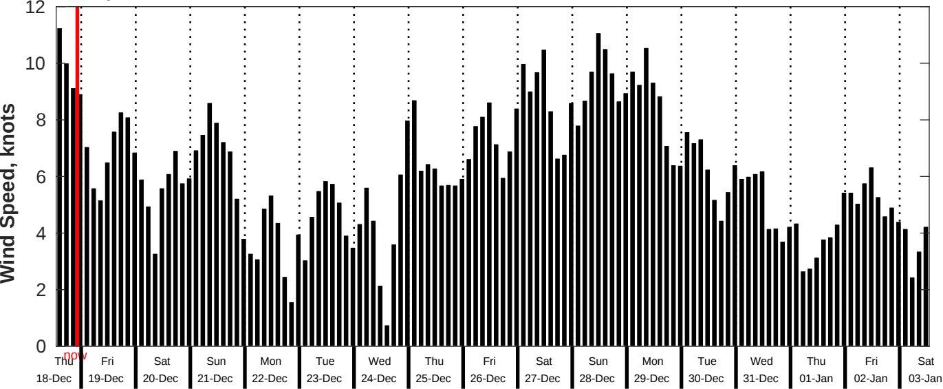
GFS Wind Speed Forecast for NDBC 51209 from 18-Dec-2025 13:00:00 to 03-Jan-2026 13:00:00
