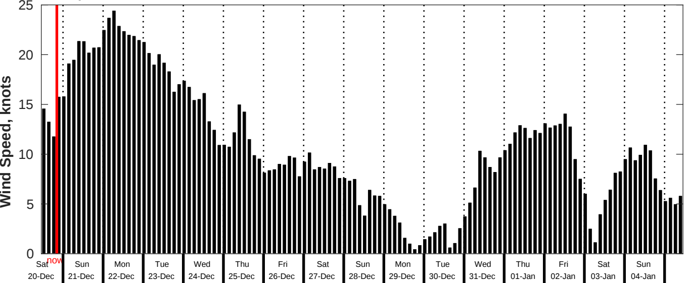
GFS Wind Speed Forecast for NDBC 52211 from 19-Dec-2025 11:00:00 to 04-Jan-2026 11:00:00
