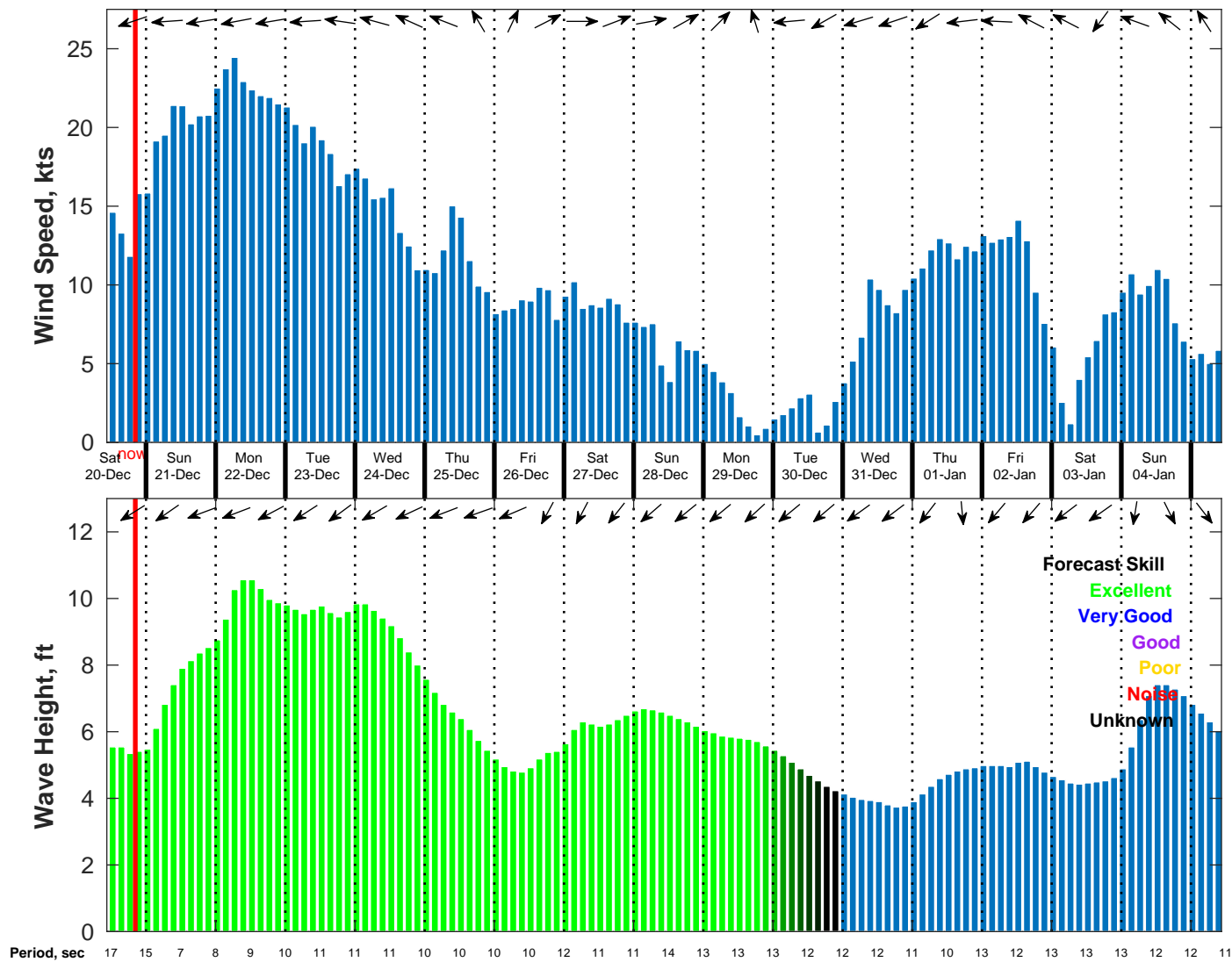
Wind & Wave Forecast for NDBC 52211 from 19-Dec-2025 11:00:00 to 04-Jan-2026 11:00:00
