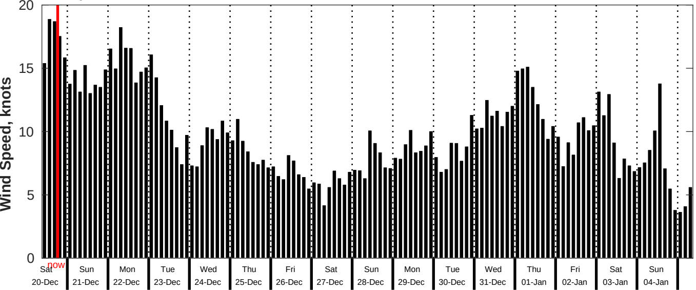
GFS Wind Speed Forecast for NDBC 52212 from 19-Dec-2025 09:00:00 to 04-Jan-2026 09:00:00
