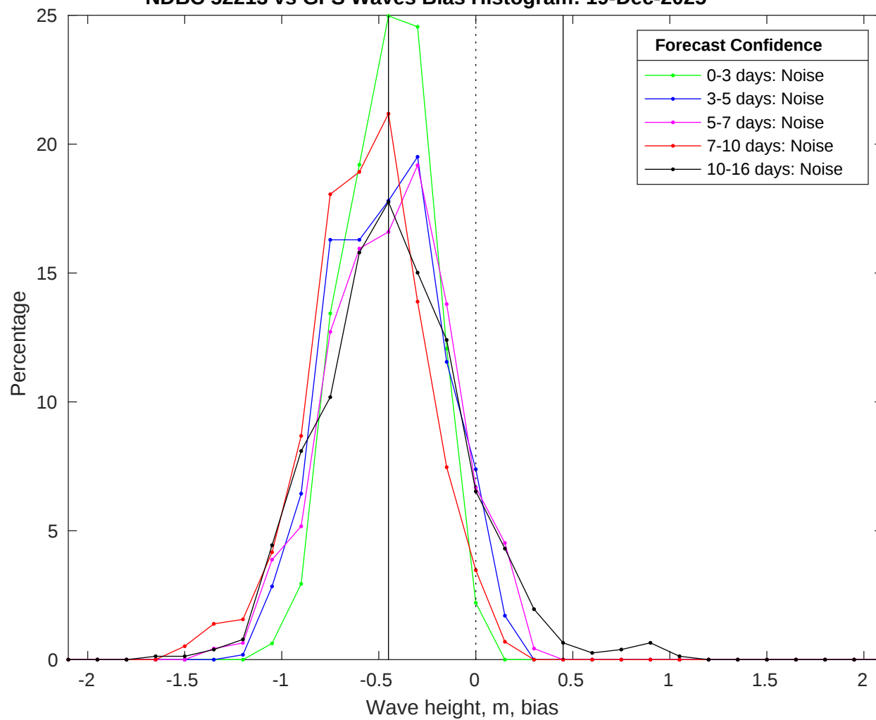
NDBC 52213 vs GFS Waves Bias Histogram: 19-Dec-2025
