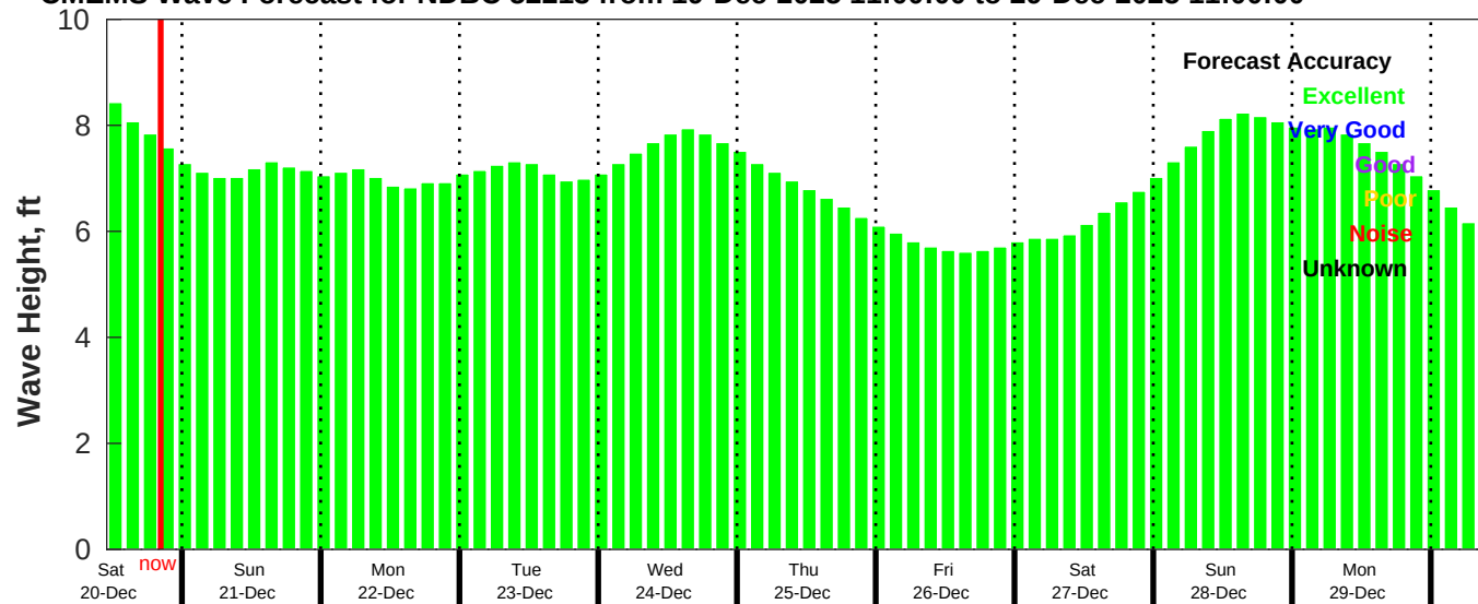
CMEMS Wave Forecast for NDBC 52213 from 19-Dec-2025 11:00:00 to 29-Dec-2025 11:00:00
