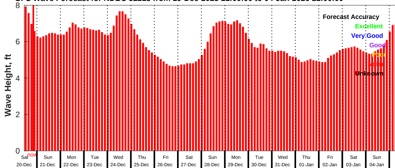
GFS Wave Forecast for NDBC 52213 from 19-Dec-2025 11:00:00 to 04-Jan-2026 11:00:00
