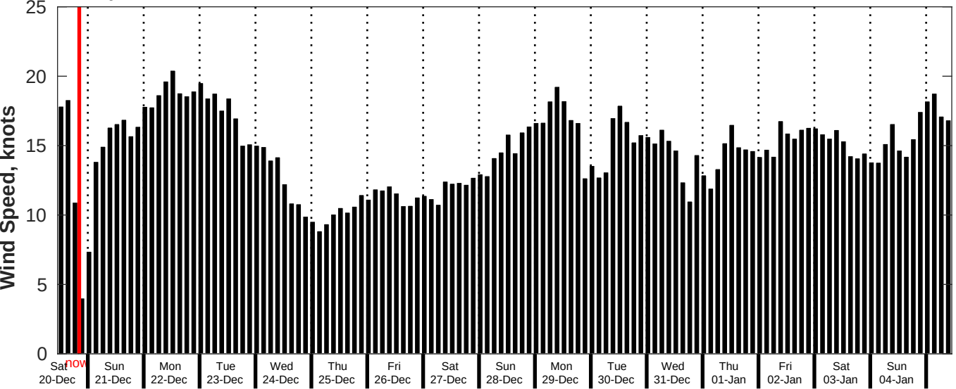
GFS Wind Speed Forecast for NDBC 52213 from 19-Dec-2025 11:00:00 to 04-Jan-2026 11:00:00
