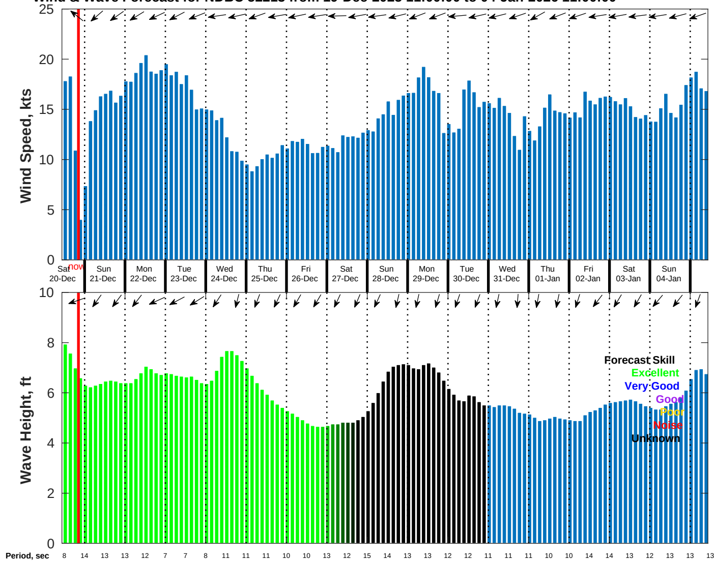
Wind & Wave Forecast for NDBC 52213 from 19-Dec-2025 11:00:00 to 04-Jan-2026 11:00:00
