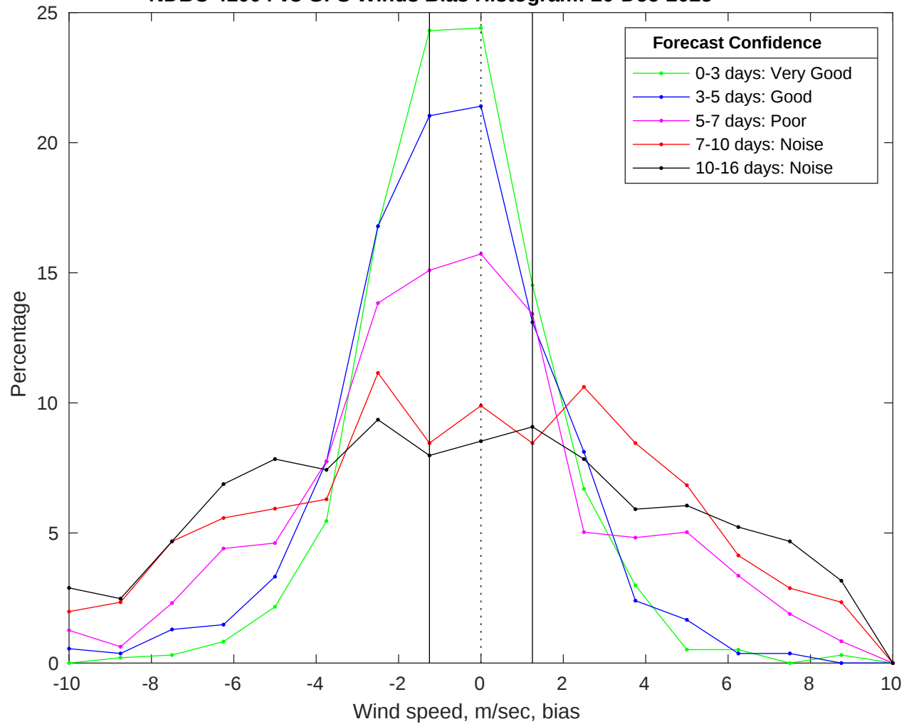
NDBC 41004 vs GFS Winds Bias Histogram: 20-Dec-2025
