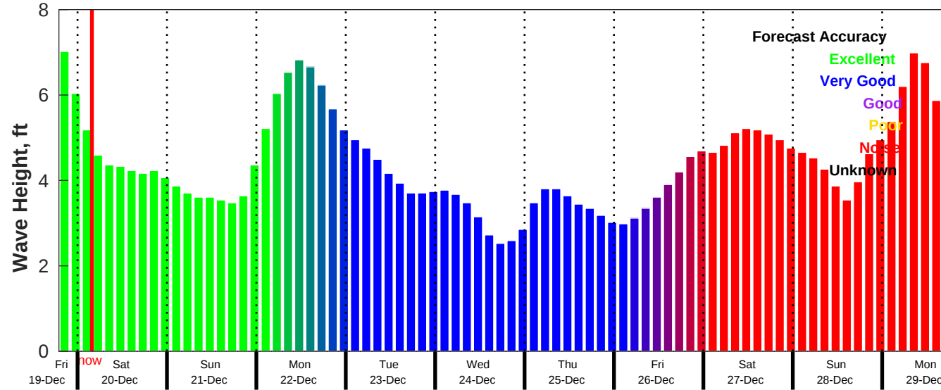
CMEMS Wave Forecast for NDBC 41004 from 19-Dec-2025 19:00:00 to 29-Dec-2025 19:00:00
