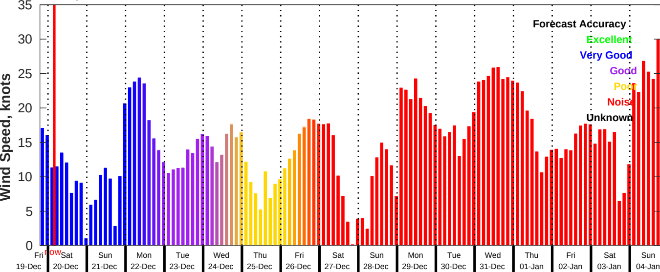
GFS Wind Speed Forecast for NDBC 41004 from 19-Dec-2025 19:00:00 to 04-Jan-2026 19:00:00
