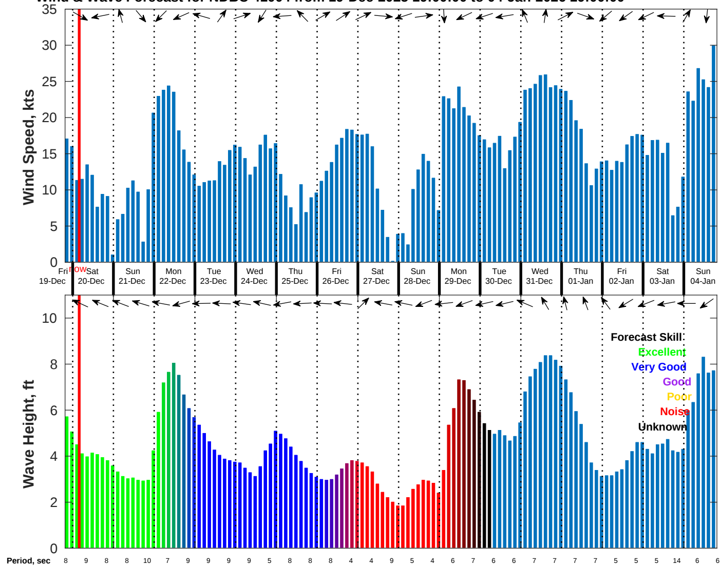
Wind & Wave Forecast for NDBC 41004 from 19-Dec-2025 19:00:00 to 04-Jan-2026 19:00:00
