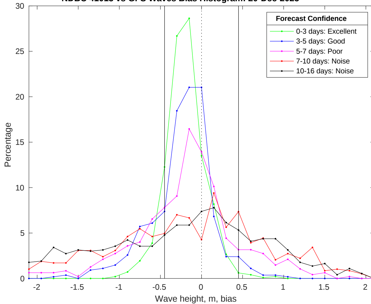
NDBC 41013 vs GFS Waves Bias Histogram: 20-Dec-2025
