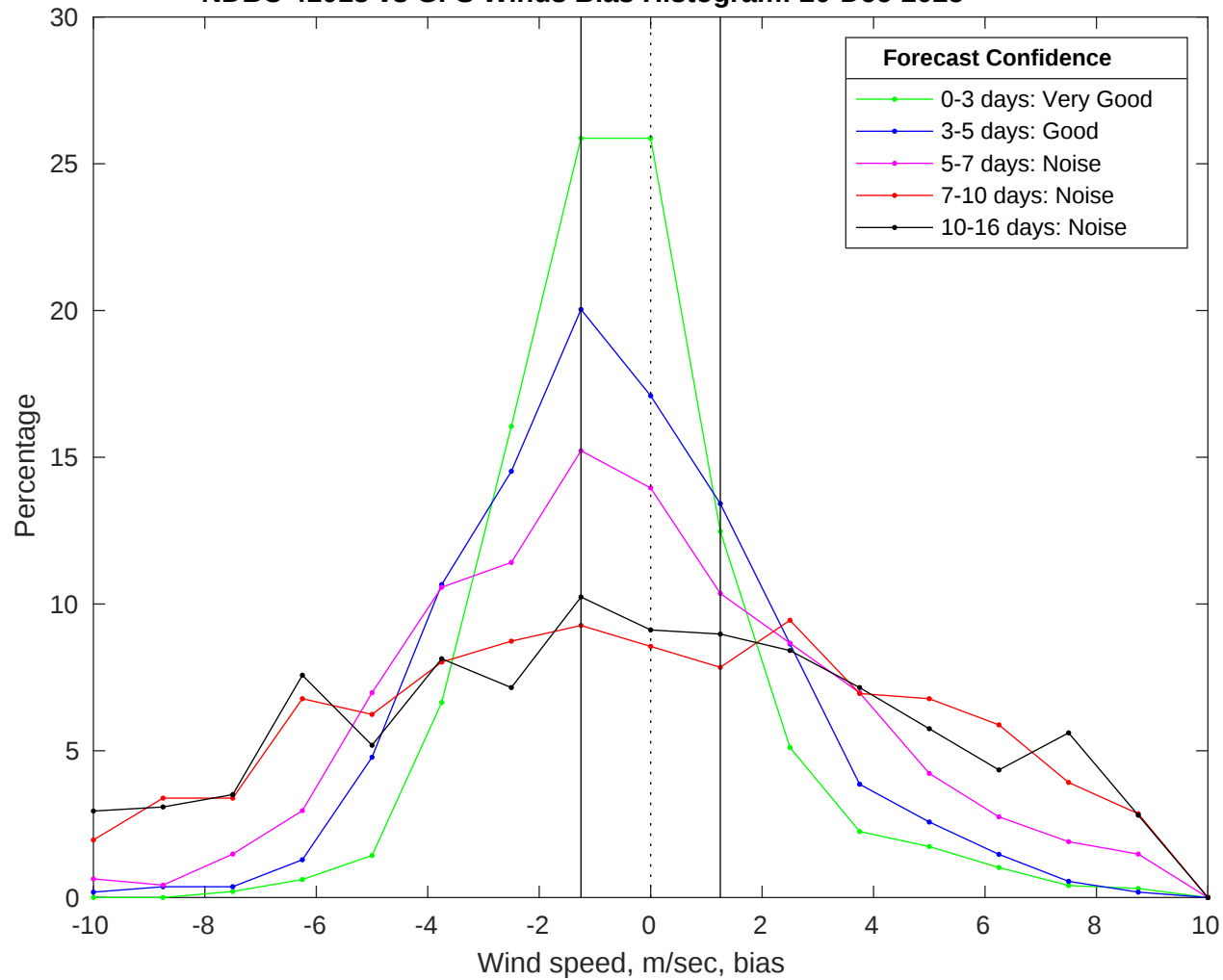
NDBC 41013 vs GFS Winds Bias Histogram: 20-Dec-2025
