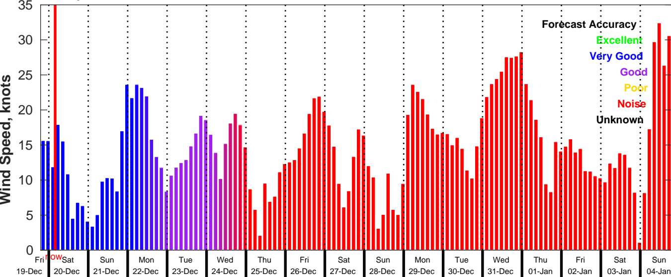
GFS Wind Speed Forecast for NDBC 41013 from 19-Dec-2025 19:00:00 to 04-Jan-2026 19:00:00
