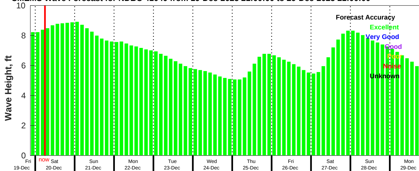
CMEMS Wave Forecast for NDBC 41040 from 19-Dec-2025 21:00:00 to 29-Dec-2025 21:00:00
