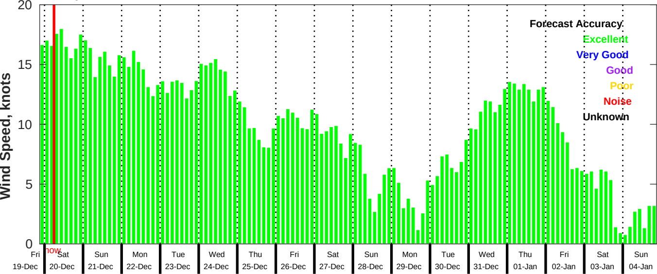
GFS Wind Speed Forecast for NDBC 41040 from 19-Dec-2025 21:00:00 to 04-Jan-2026 21:00:00
