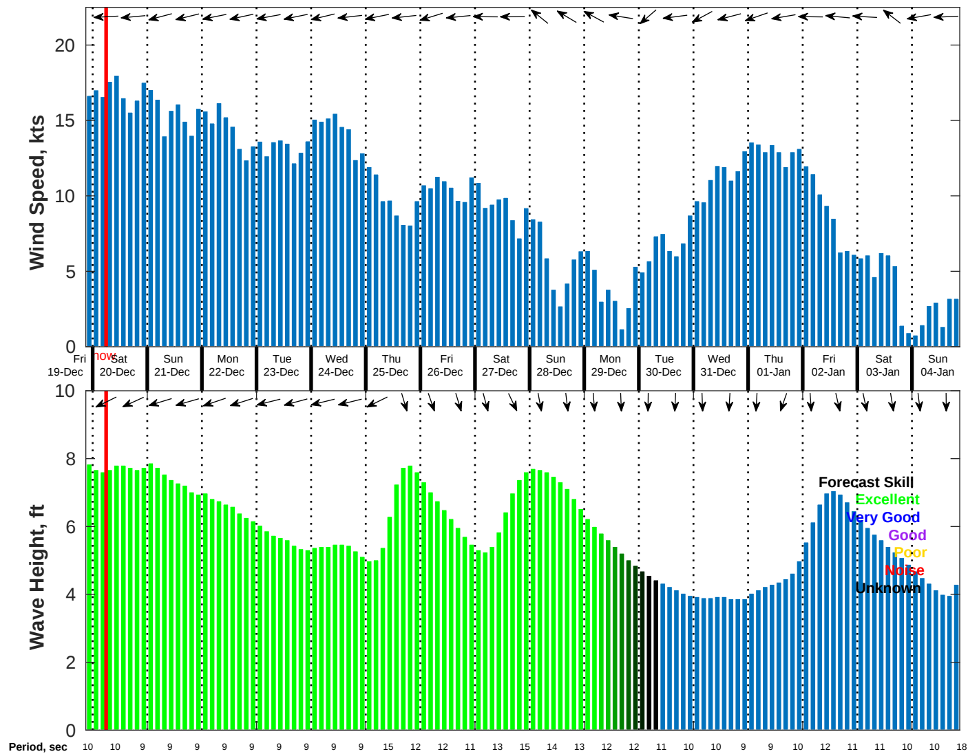
Wind & Wave Forecast for NDBC 41040 from 19-Dec-2025 21:00:00 to 04-Jan-2026 21:00:00
