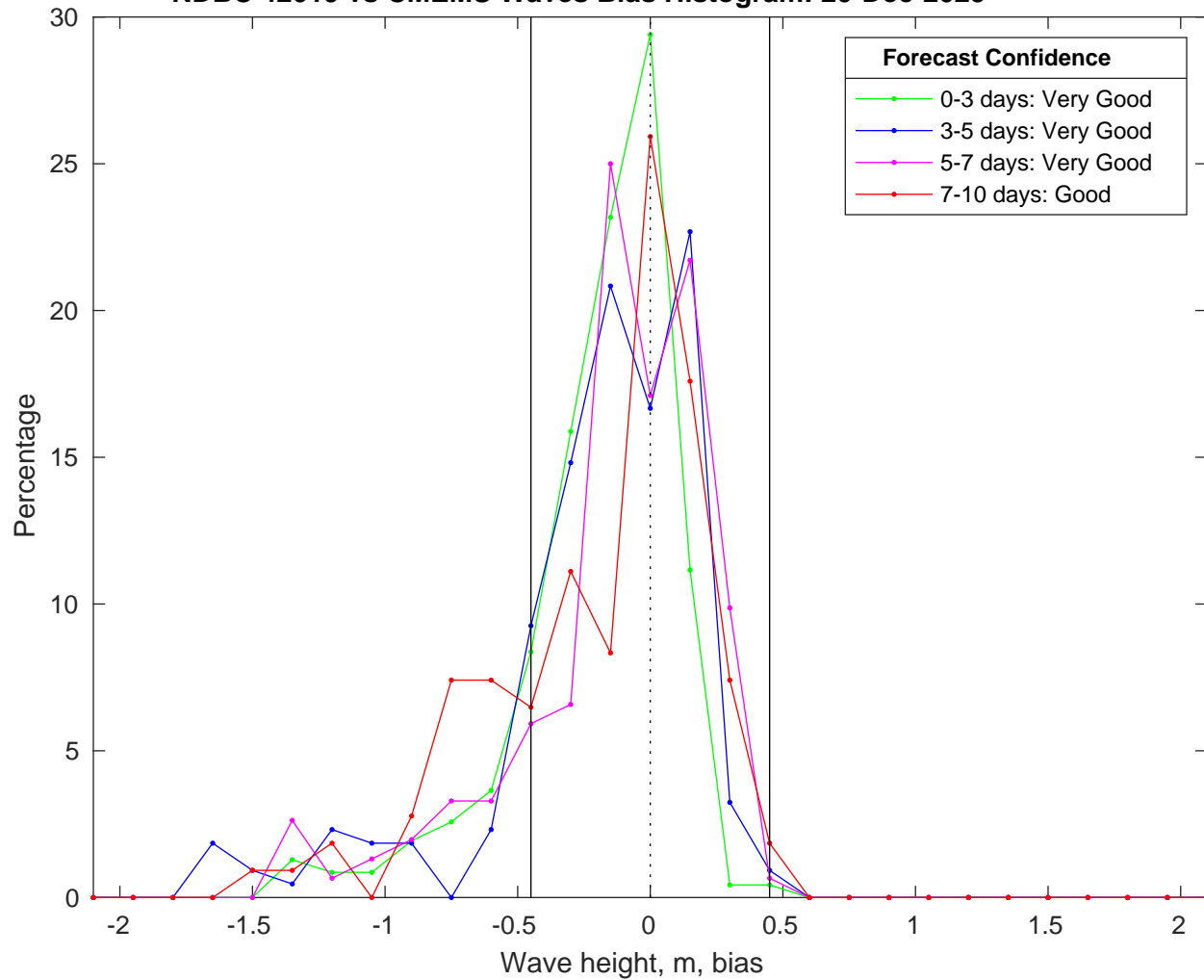
NDBC 42019 vs CMEMS Waves Bias Histogram: 20-Dec-2025
