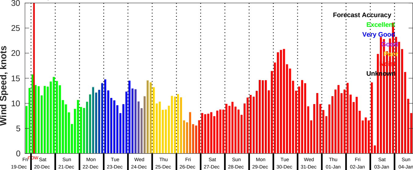
GFS Wind Speed Forecast for NDBC 42019 from 19-Dec-2025 18:00:00 to 04-Jan-2026 18:00:00
