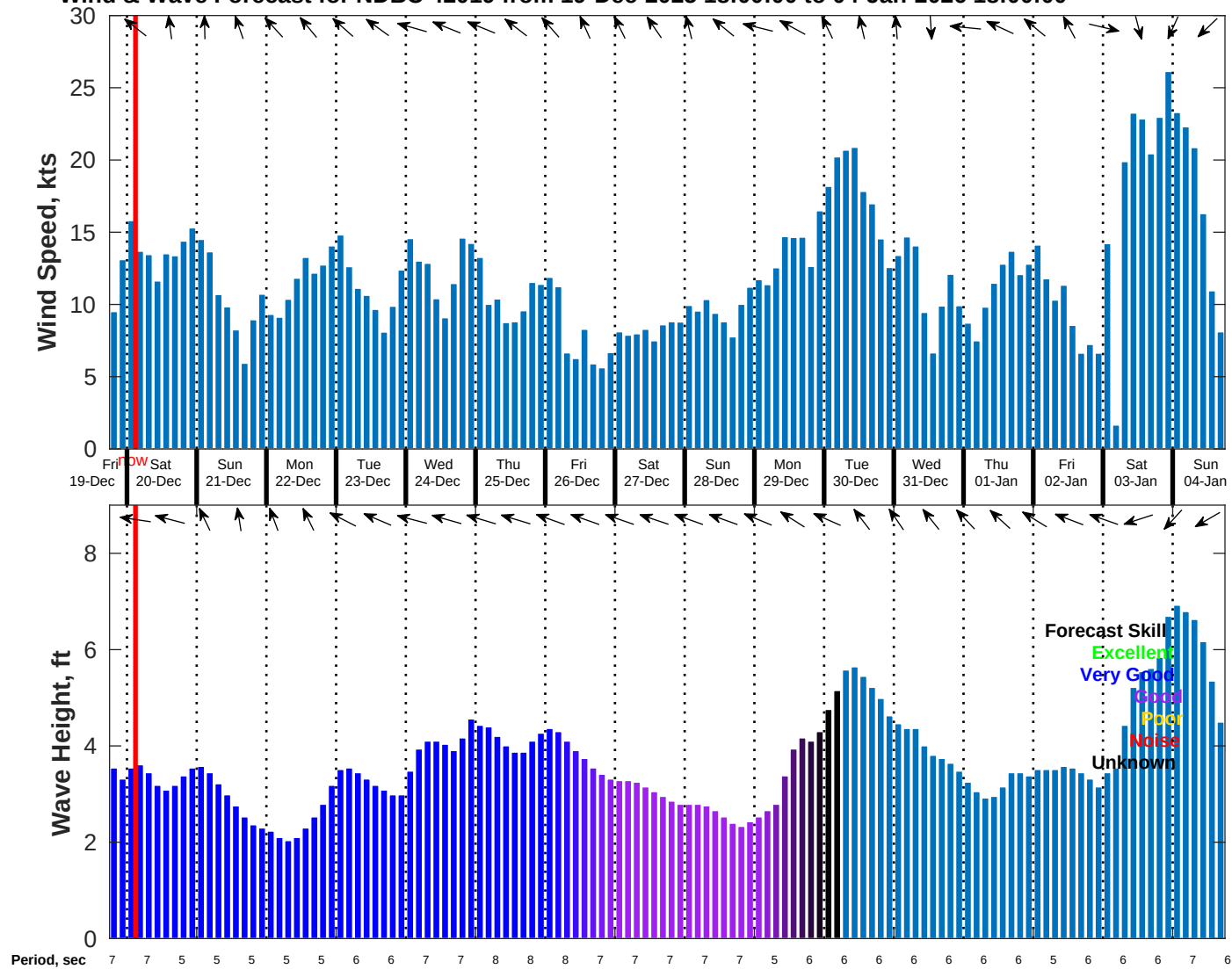
Wind & Wave Forecast for NDBC 42019 from 19-Dec-2025 18:00:00 to 04-Jan-2026 18:00:00
