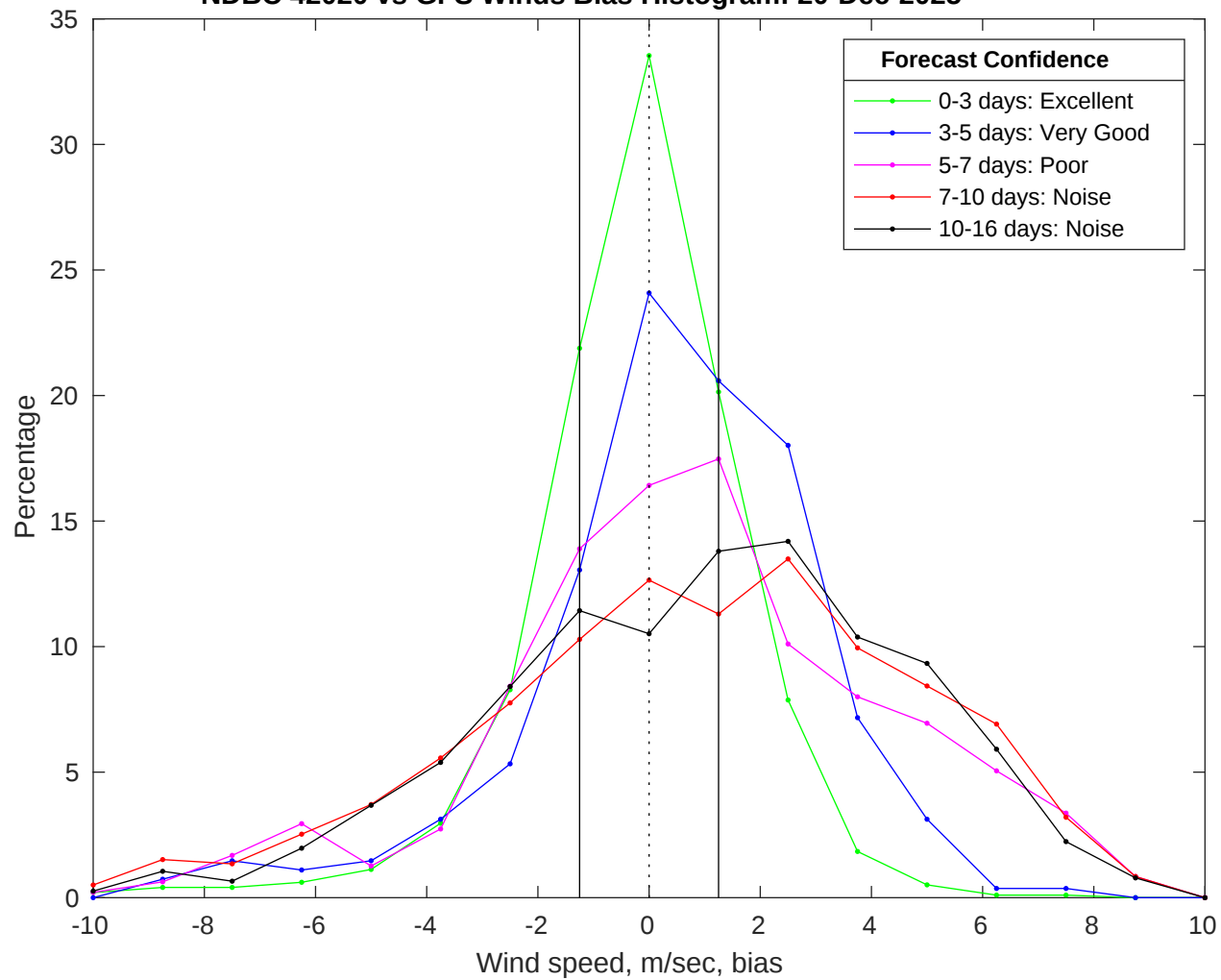
NDBC 42020 vs GFS Winds Bias Histogram: 20-Dec-2025
