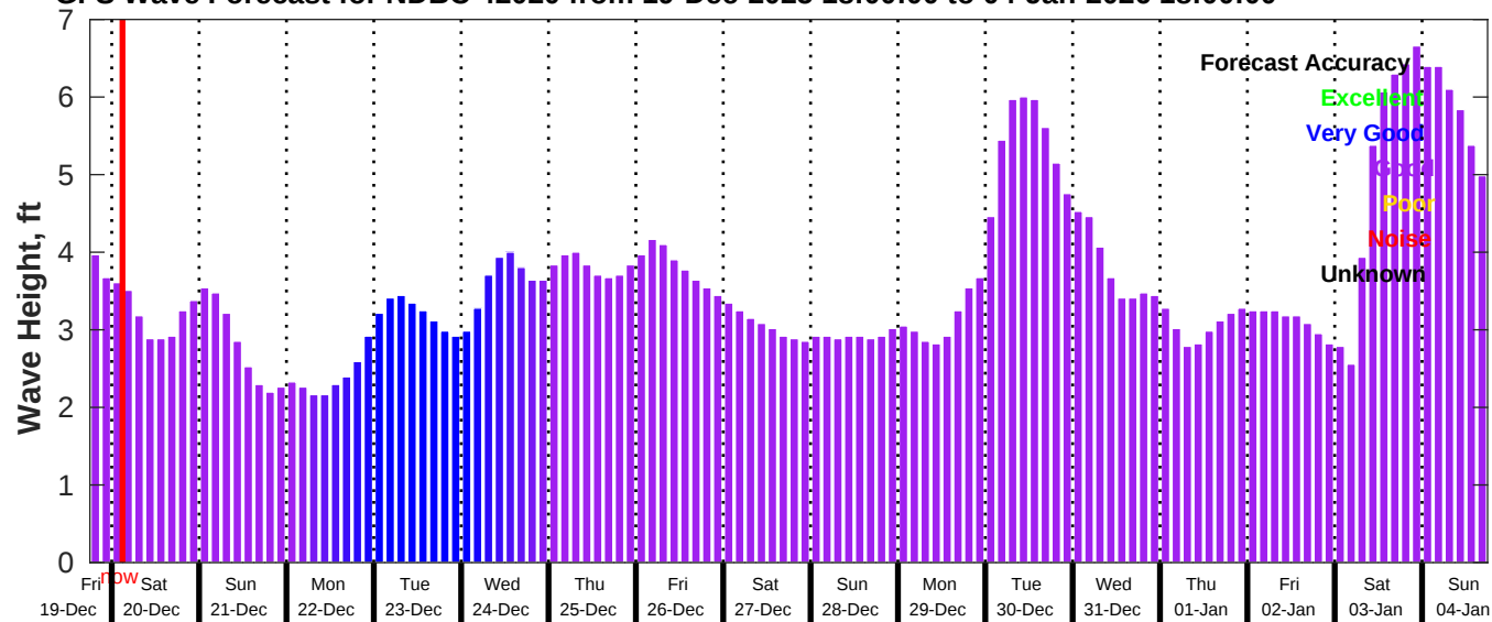
GFS Wave Forecast for NDBC 42020 from 19-Dec-2025 18:00:00 to 04-Jan-2026 18:00:00
