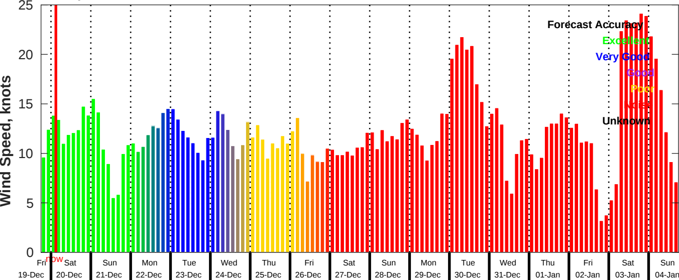
GFS Wind Speed Forecast for NDBC 42020 from 19-Dec-2025 18:00:00 to 04-Jan-2026 18:00:00
