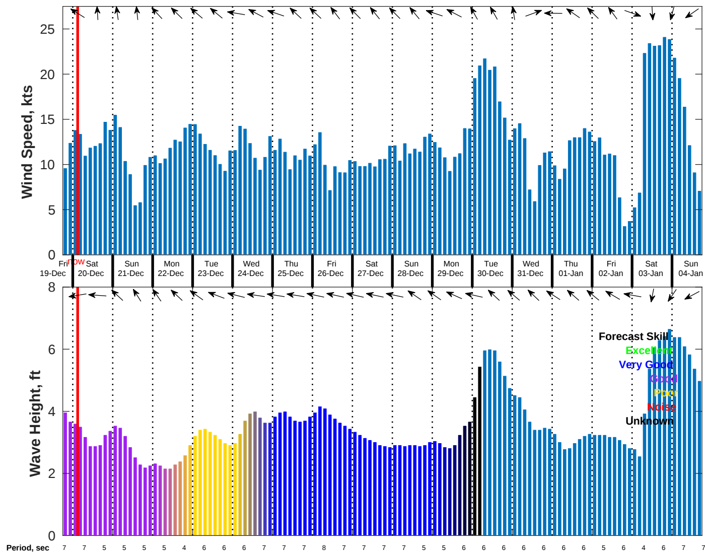
Wind & Wave Forecast for NDBC 42020 from 19-Dec-2025 18:00:00 to 04-Jan-2026 18:00:00
