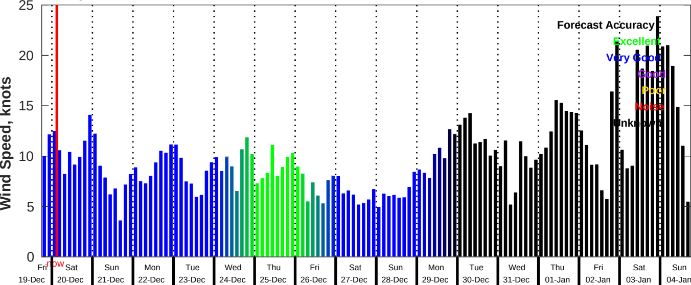
GFS Wind Speed Forecast for NDBC 42035 from 19-Dec-2025 18:00:00 to 04-Jan-2026 18:00:00
