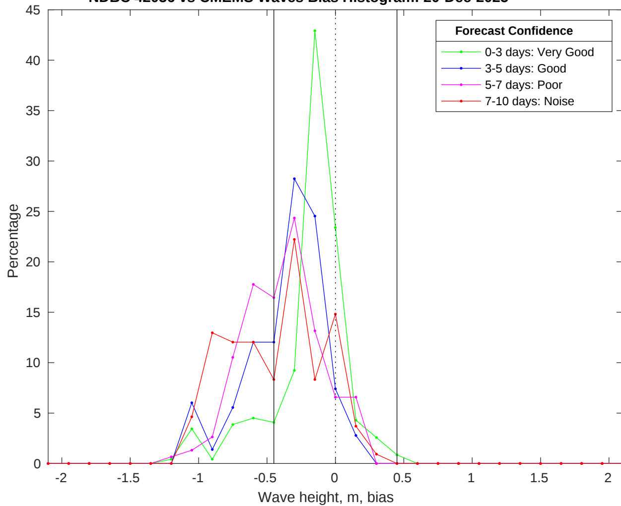
NDBC 42036 vs CMEMS Waves Bias Histogram: 20-Dec-2025
