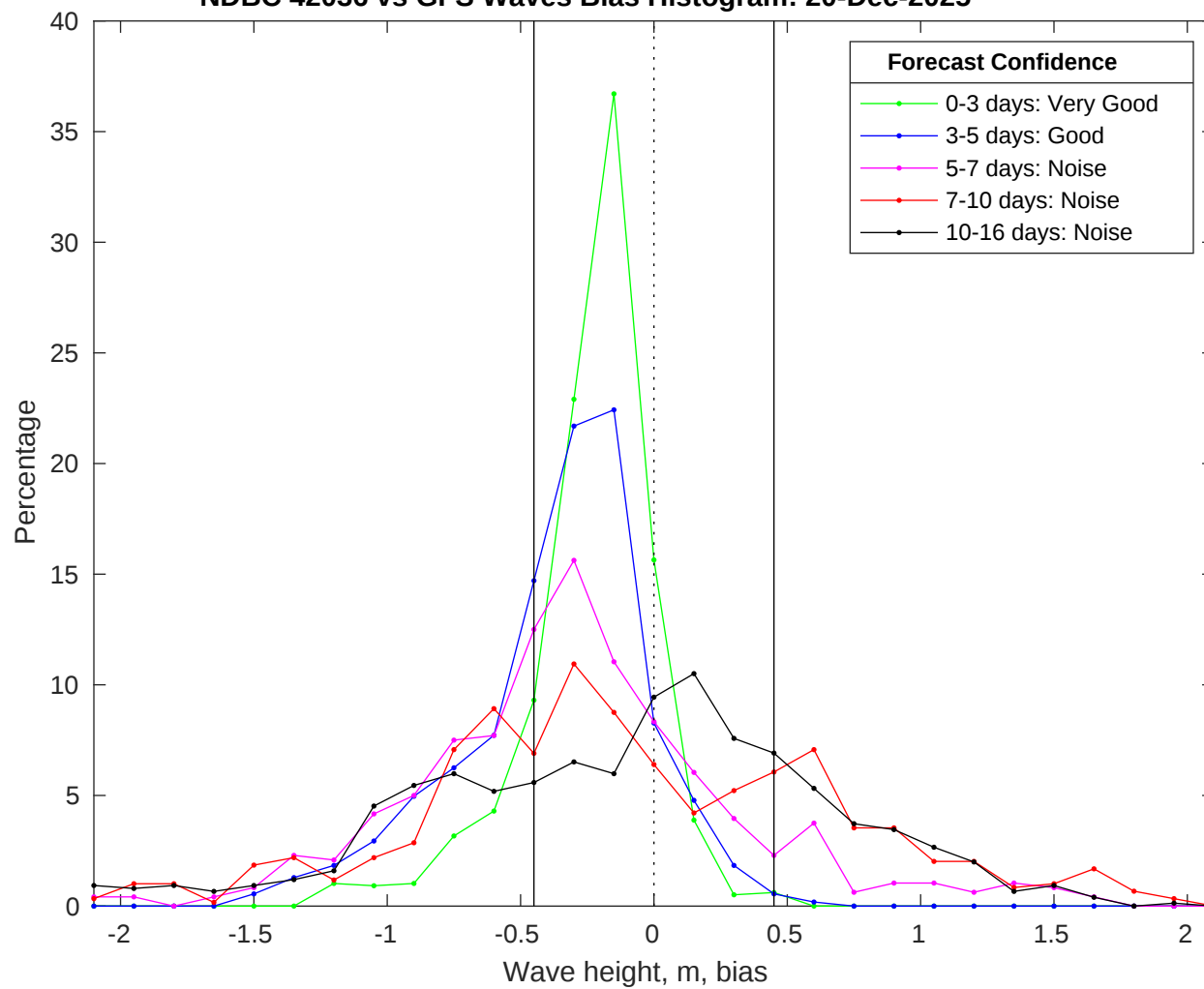
NDBC 42036 vs GFS Waves Bias Histogram: 20-Dec-2025
