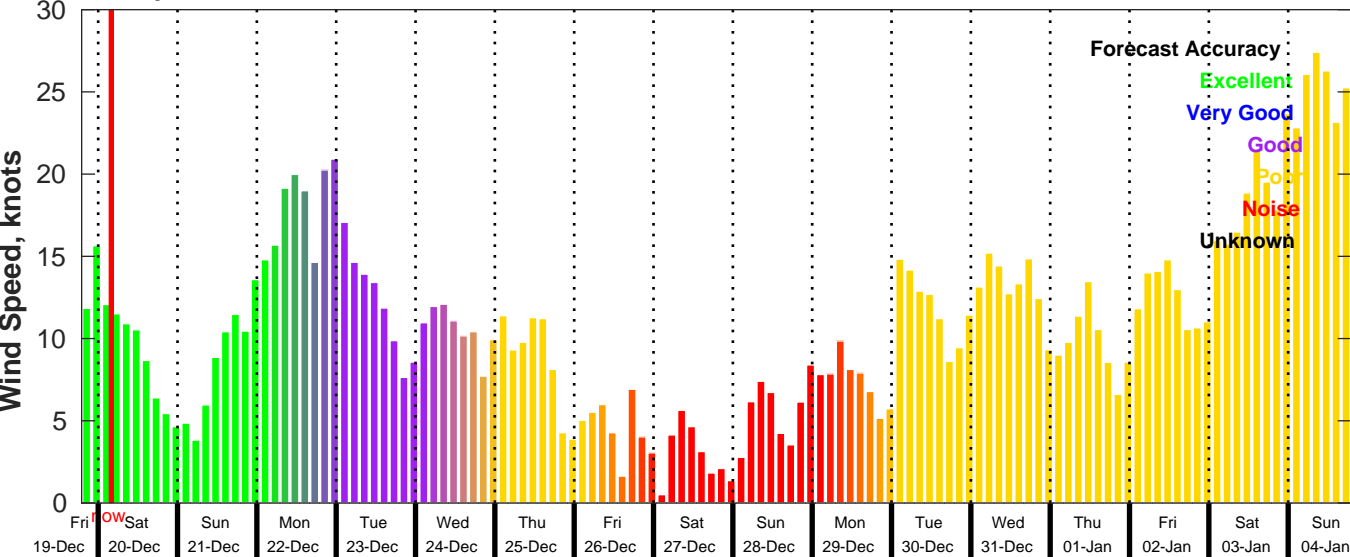
GFS Wind Speed Forecast for NDBC 42036 from 19-Dec-2025 19:00:00 to 04-Jan-2026 19:00:00
