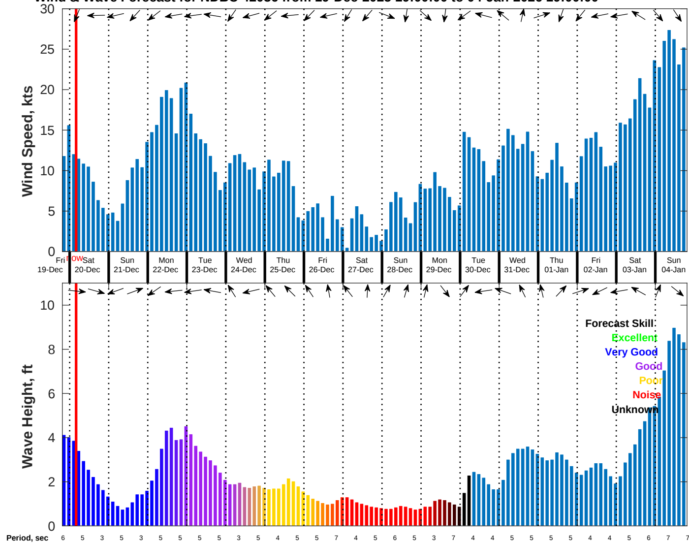
Wind & Wave Forecast for NDBC 42036 from 19-Dec-2025 19:00:00 to 04-Jan-2026 19:00:00
