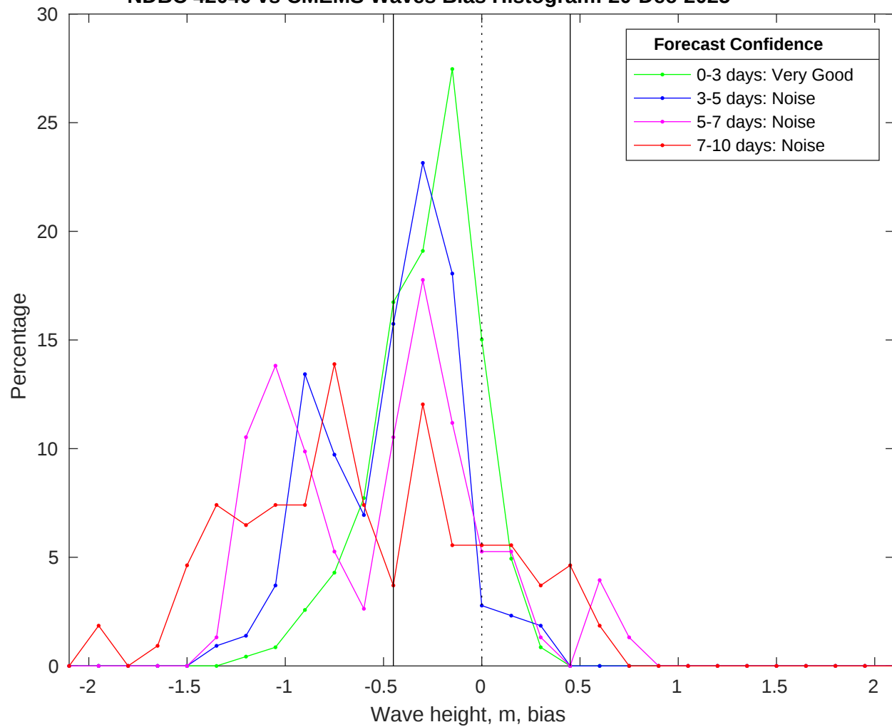
NDBC 42040 vs CMEMS Waves Bias Histogram: 20-Dec-2025
