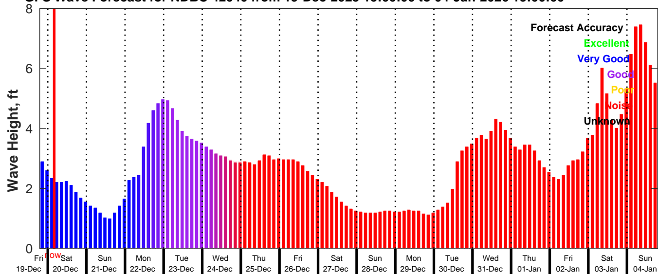
GFS Wave Forecast for NDBC 42040 from 19-Dec-2025 19:00:00 to 04-Jan-2026 19:00:00
