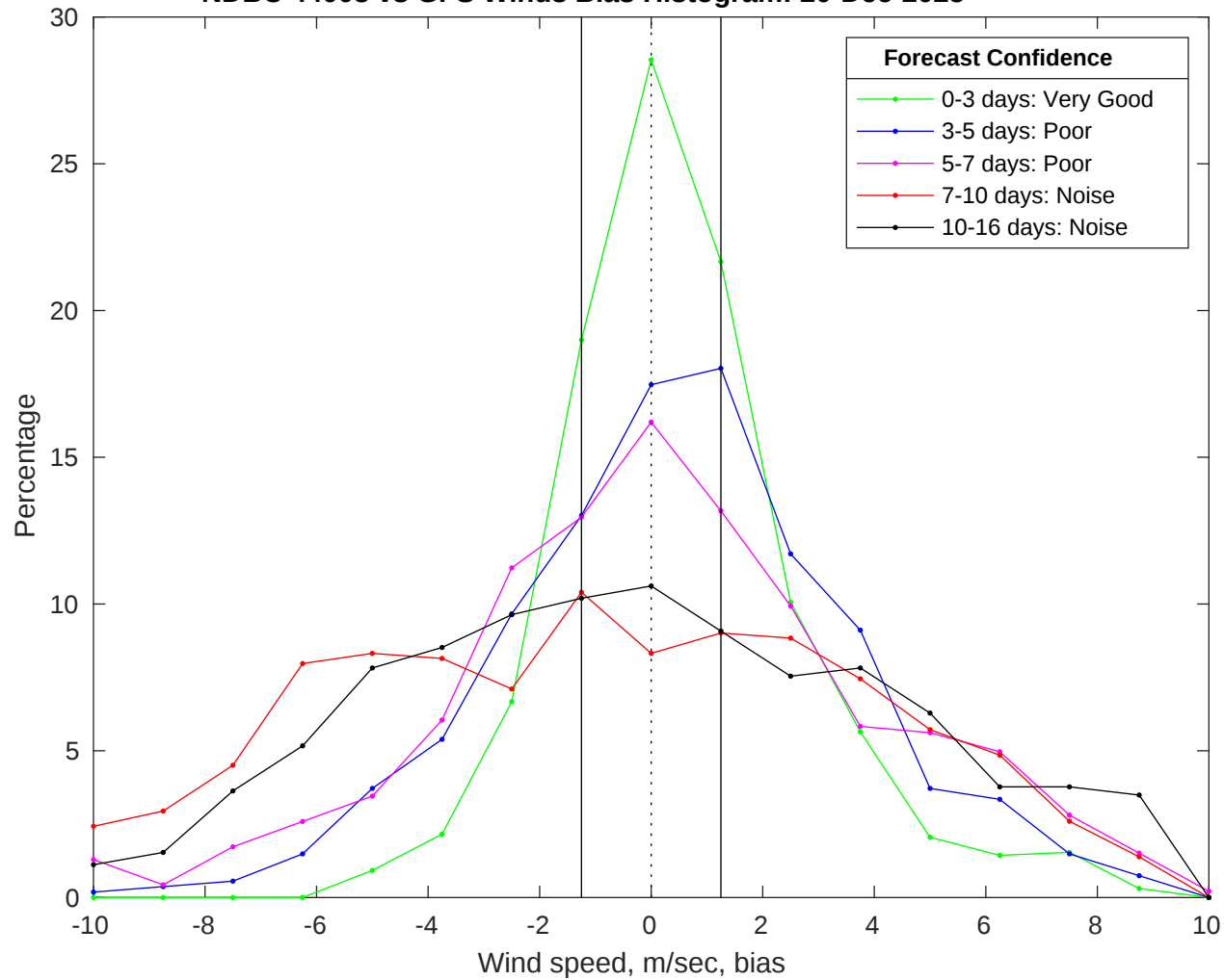
NDBC 44008 vs GFS Winds Bias Histogram: 20-Dec-2025
