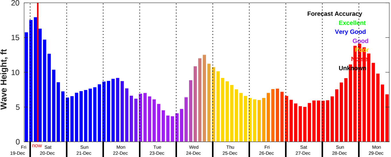
CMEMS Wave Forecast for NDBC 44008 from 19-Dec-2025 20:00:00 to 29-Dec-2025 20:00:00
