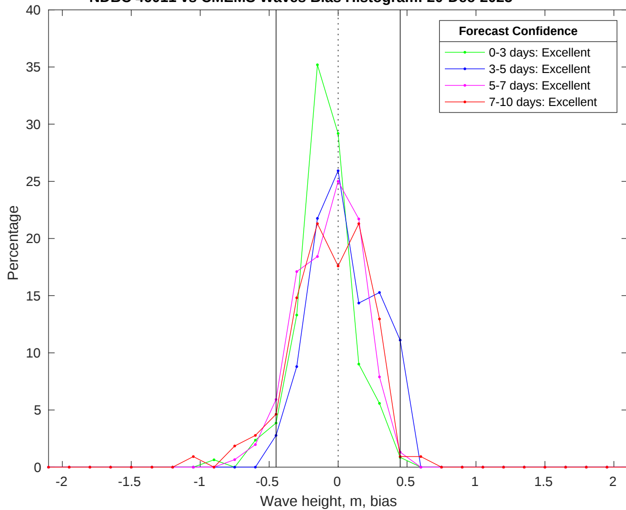
NDBC 46011 vs CMEMS Waves Bias Histogram: 20-Dec-2025
