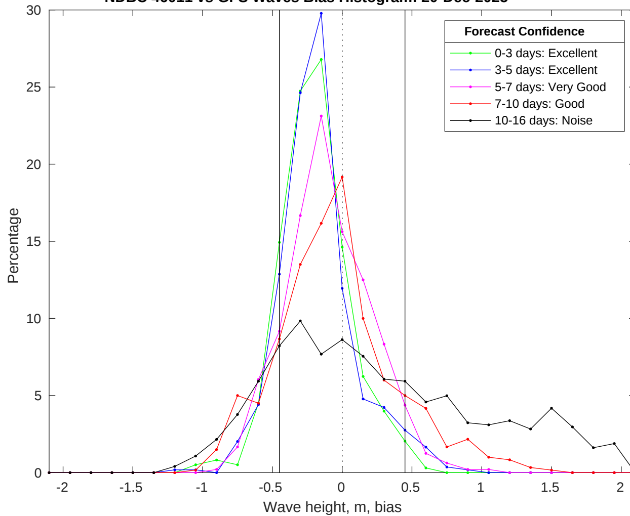
NDBC 46011 vs GFS Waves Bias Histogram: 20-Dec-2025
