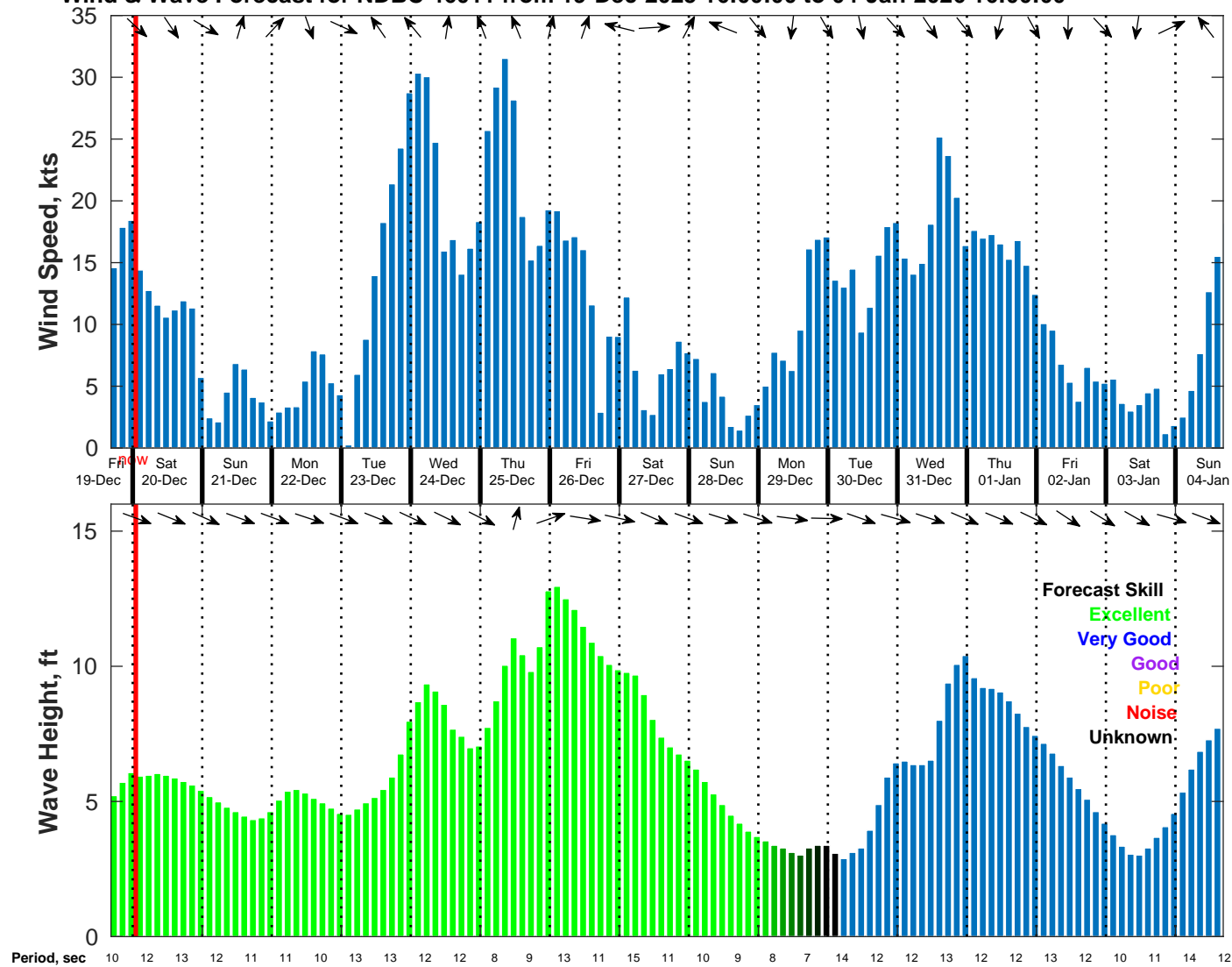
Wind & Wave Forecast for NDBC 46011 from 19-Dec-2025 16:00:00 to 04-Jan-2026 16:00:00
