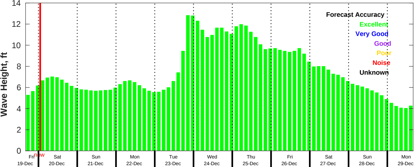
CMEMS Wave Forecast for NDBC 46028 from 19-Dec-2025 16:00:00 to 29-Dec-2025 16:00:00
