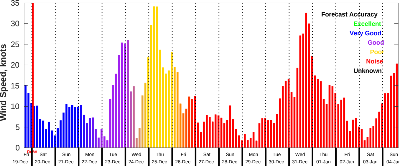
GFS Wind Speed Forecast for NDBC 46028 from 19-Dec-2025 16:00:00 to 04-Jan-2026 16:00:00
