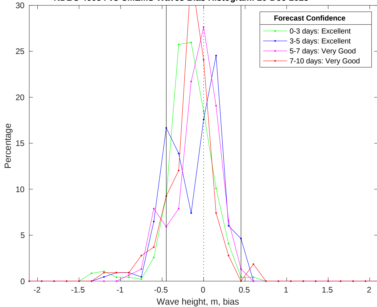
NDBC 46054 vs CMEMS Waves Bias Histogram: 20-Dec-2025
