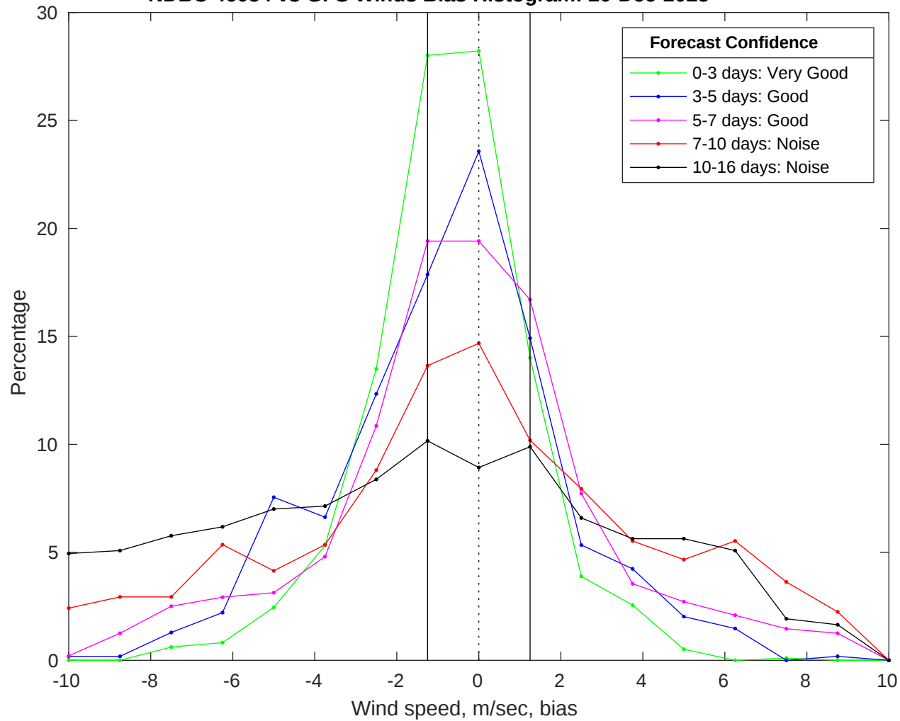
NDBC 46054 vs GFS Winds Bias Histogram: 20-Dec-2025
