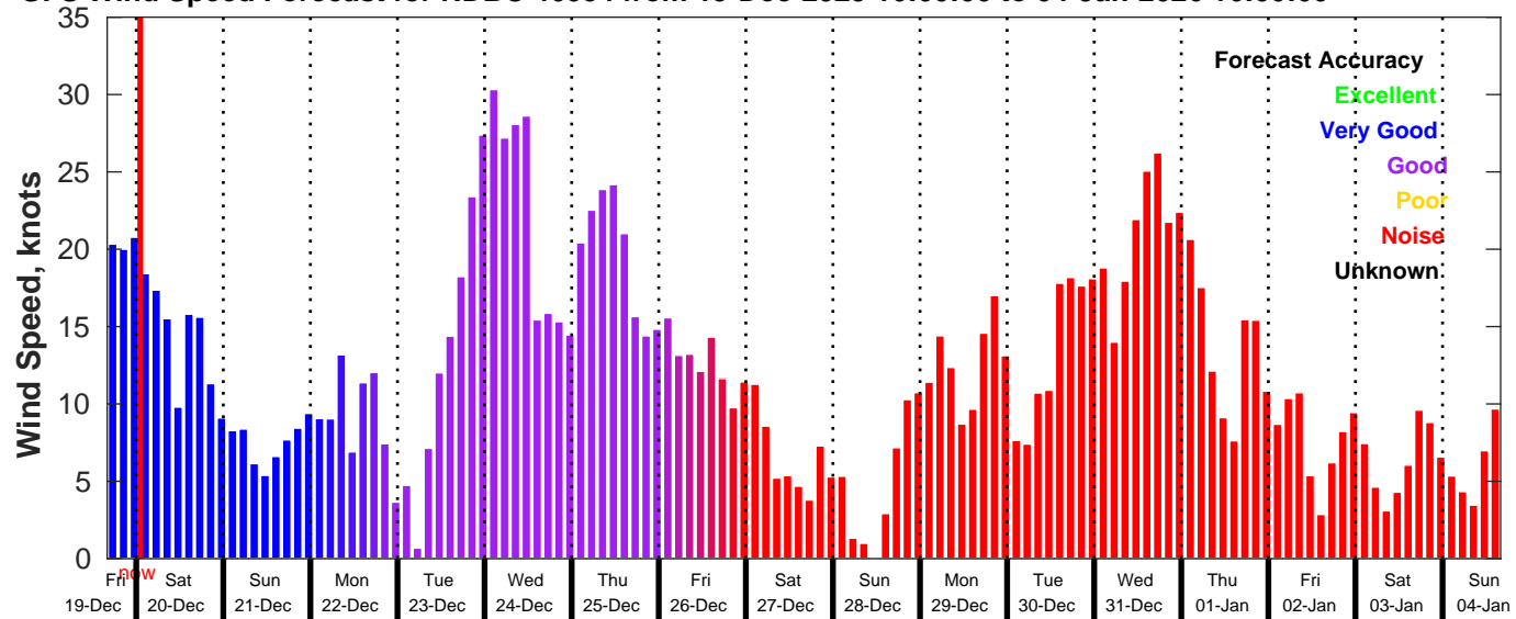
GFS Wind Speed Forecast for NDBC 46054 from 19-Dec-2025 16:00:00 to 04-Jan-2026 16:00:00
